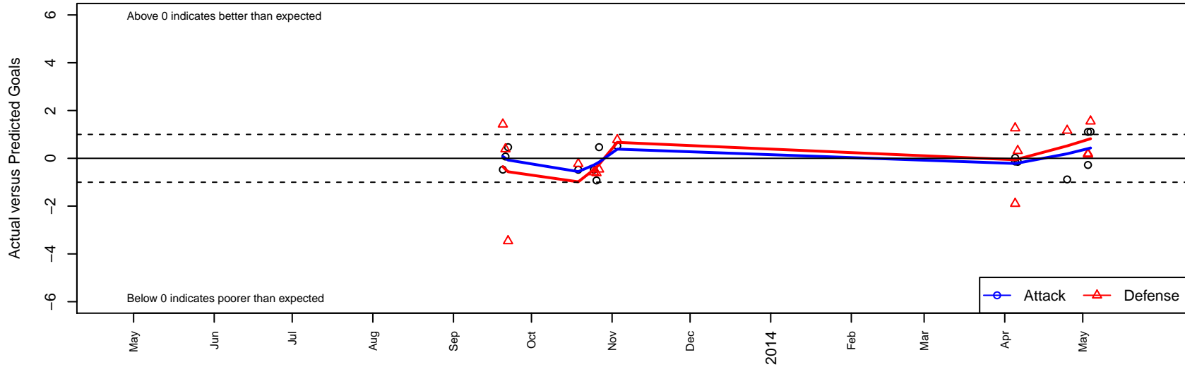
SLSG ECNL G99 Dots are actual minus expected GF (blue circles) and GA (red triangles). Blue line is smoothed change in attack strength. Red is smoothed change in defense strength.
